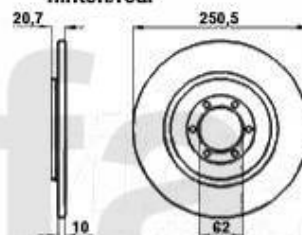
5. 610 118415 Turbo/V6/2.4TD hinten/rear
